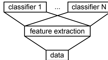
Fig. 1. Example for a multilingual architecture for speech recognition with a language-independent feature extraction and language-specific classifiers on top of it.
